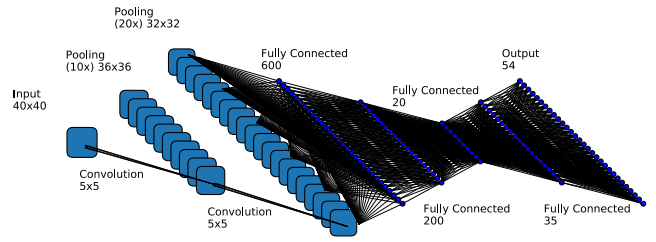
Fig. 3: The image-to-motion encoder-decoder network (CIMEDNet) at the core of the overall architecture shown in Fig. 2 with an encoder consisting of two convolutional layers followed by two fully-connected layers, and a decoder consisting of three fully-connected layers.
