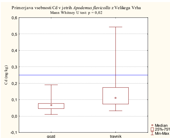
Fig. 2: Comparisons between Hg and Cd levels in forest and meadow soil and in liver of Apodemus flavicollis , collected in the forest and meadow research area. Red lines indicate limit values for Hg and Cd (Official Gazette RS, No. 68/1996). Blue lines indicate effect concentrations for small mammals according to Ma et al., 1991 and Wijnhoven et al., 2008.
